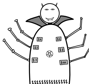
Figure 11.1 Would you play with this multi-armed bandit?
