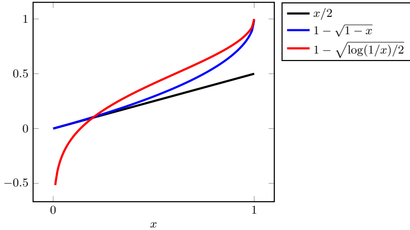
Figure 14.2 Tightening the inequality of Le Cam. Here, x = \exp(-D(P, Q)) . Higher values are better as the figure shows lower bounds on P(A) + Q(A^c) . The black curve corresponds to (14.7), the blue curve corresponds to (14.11) and the red curve corresponds to (14.12) (Pinsker’s inequality). As can be seen, (14.11) indeed dominates (14.7). Also, while for x small ( D(P, Q) large) Pinsker is vacuous, while the others are not, for x larger ( D(P, Q) near zero) Pinsker dominates (14.11), though in the limit when D(P, Q) = 0 , both Pinsker and (14.11) give the “correct” value of 1.
